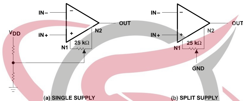
Figure 105. Input Offset Voltage Null Circuit
